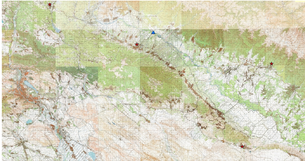
Fig 1. The location of GNIP and GNIR stations
