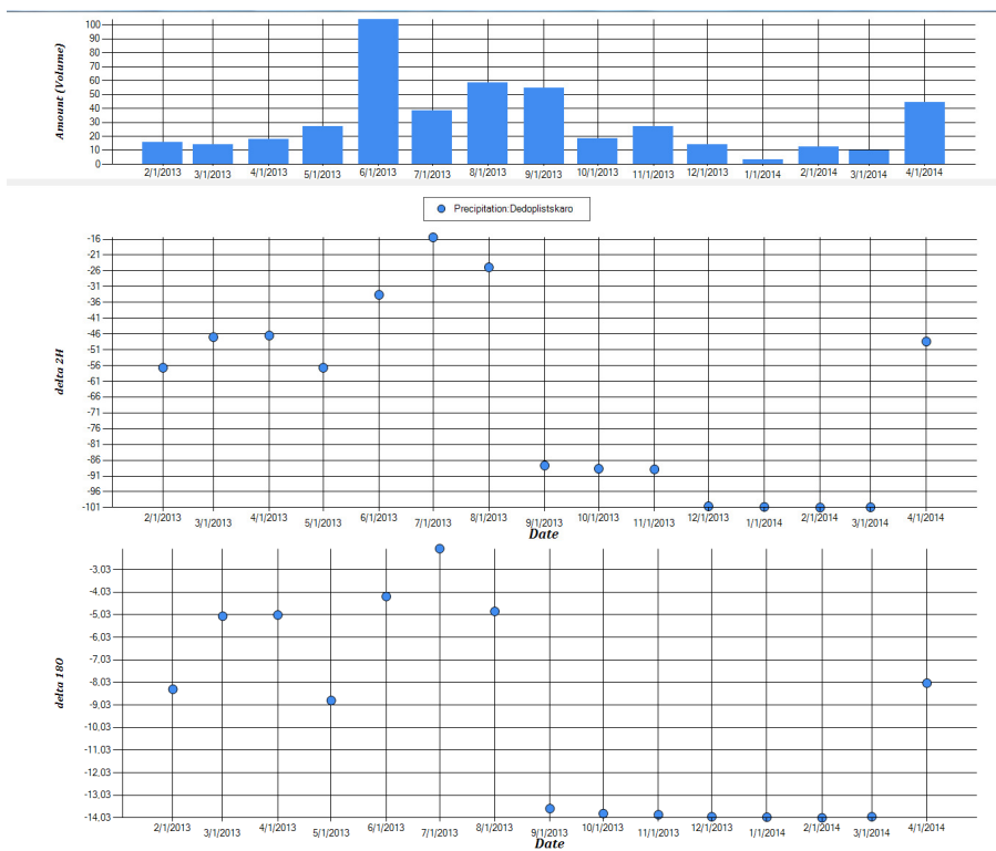
Fig. 5 Stable isotope variation in precipitation curve; “Dedoplistskaro” station
